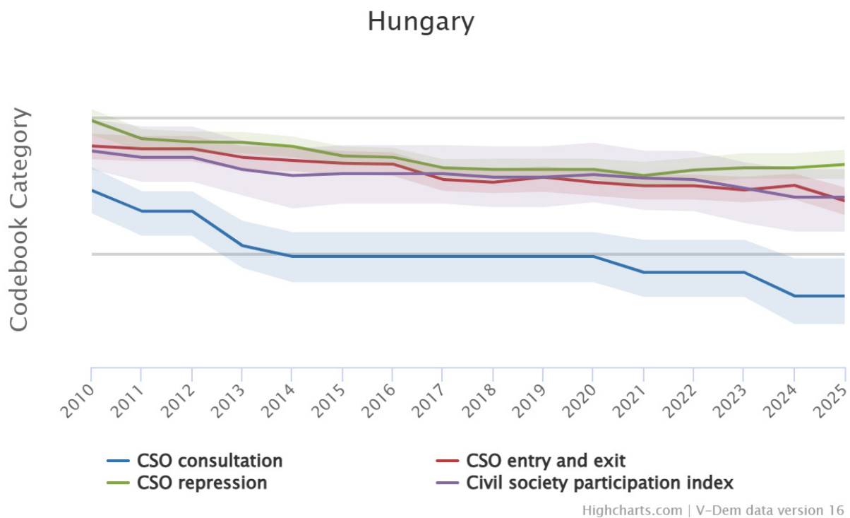
Figure 1 Hungary, civil society indicators 2010–2025. Source: V-Dem Institute (2025), Country Graph.
